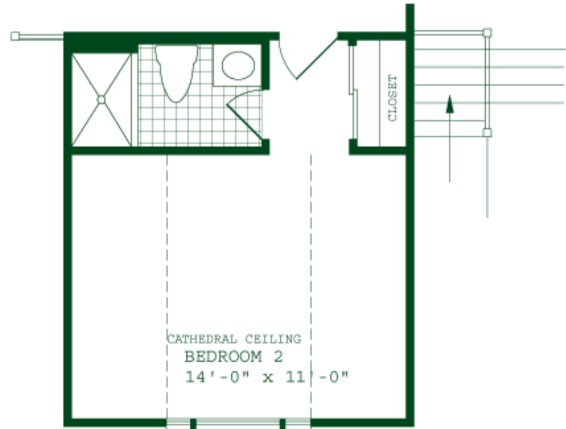
PARTIAL SECOND FLOOR PLAN SHOWING BEDROOM 2 WITH OPTIONAL BATH
